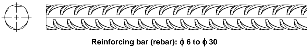
Figure 4: Steel element – ribbed reinforcing steel rod; 6 \text{ mm} \leq d \leq 30 \text{ mm}
